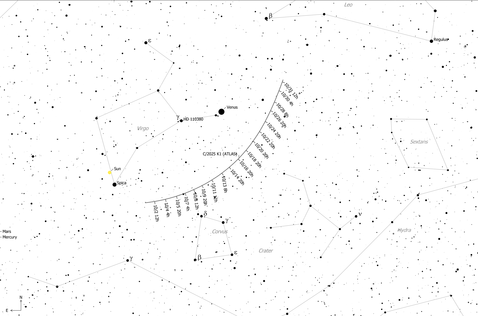
C/2025 K1 (ATLAS) (Comet) Magnitude: 9.45 Coma Diameter: 1.2' SBr: 18.4 Mag/arcsec² Earth Distance: 1.2 AU
