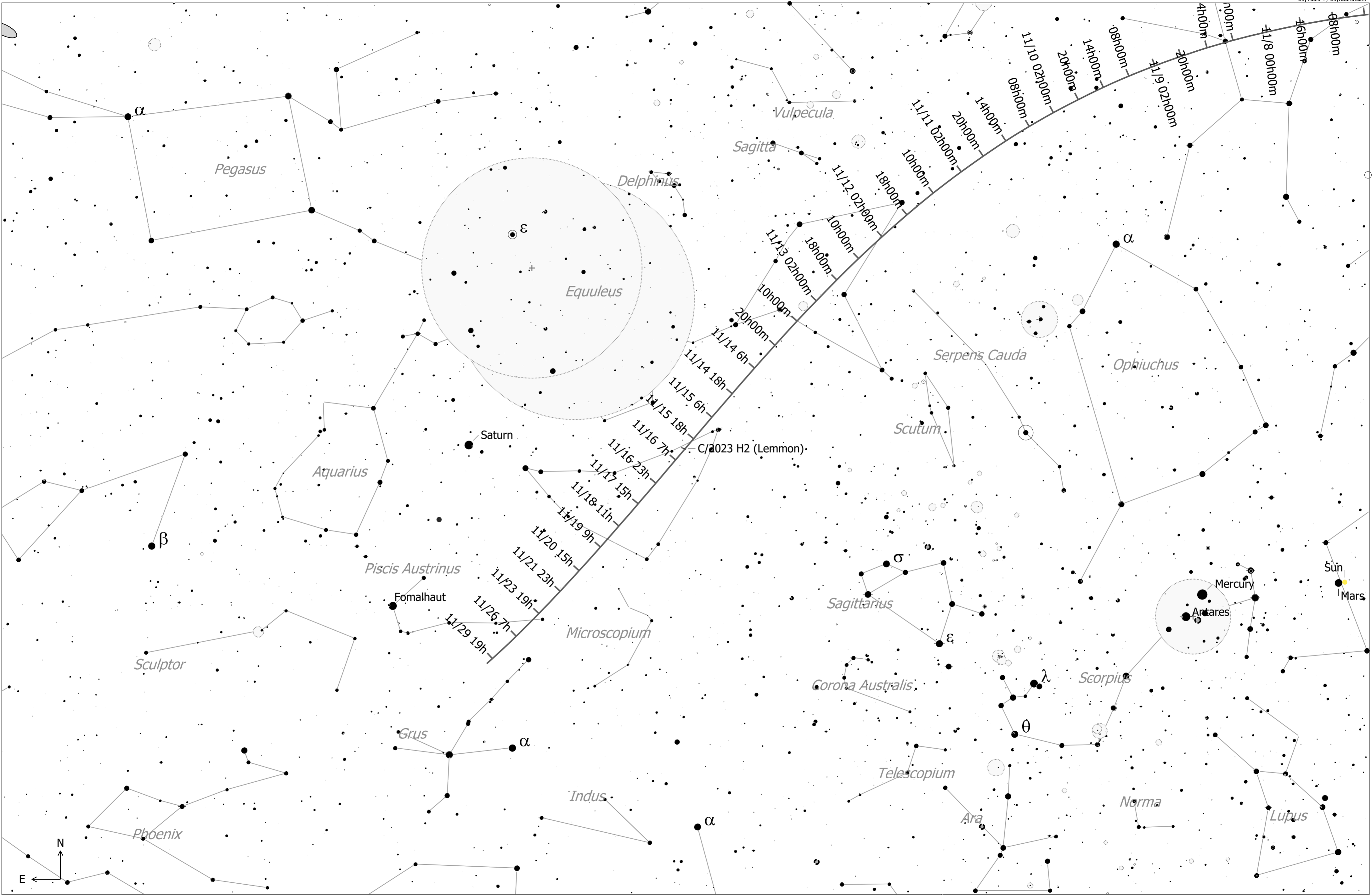
C/2023 H2 (Lemmon) (Comet) Magnitude: 7.90 Coma Diameter: 10.4' SBr: 21.6 Mag/arcsec 2 Earth Distance: 0.3 AU
