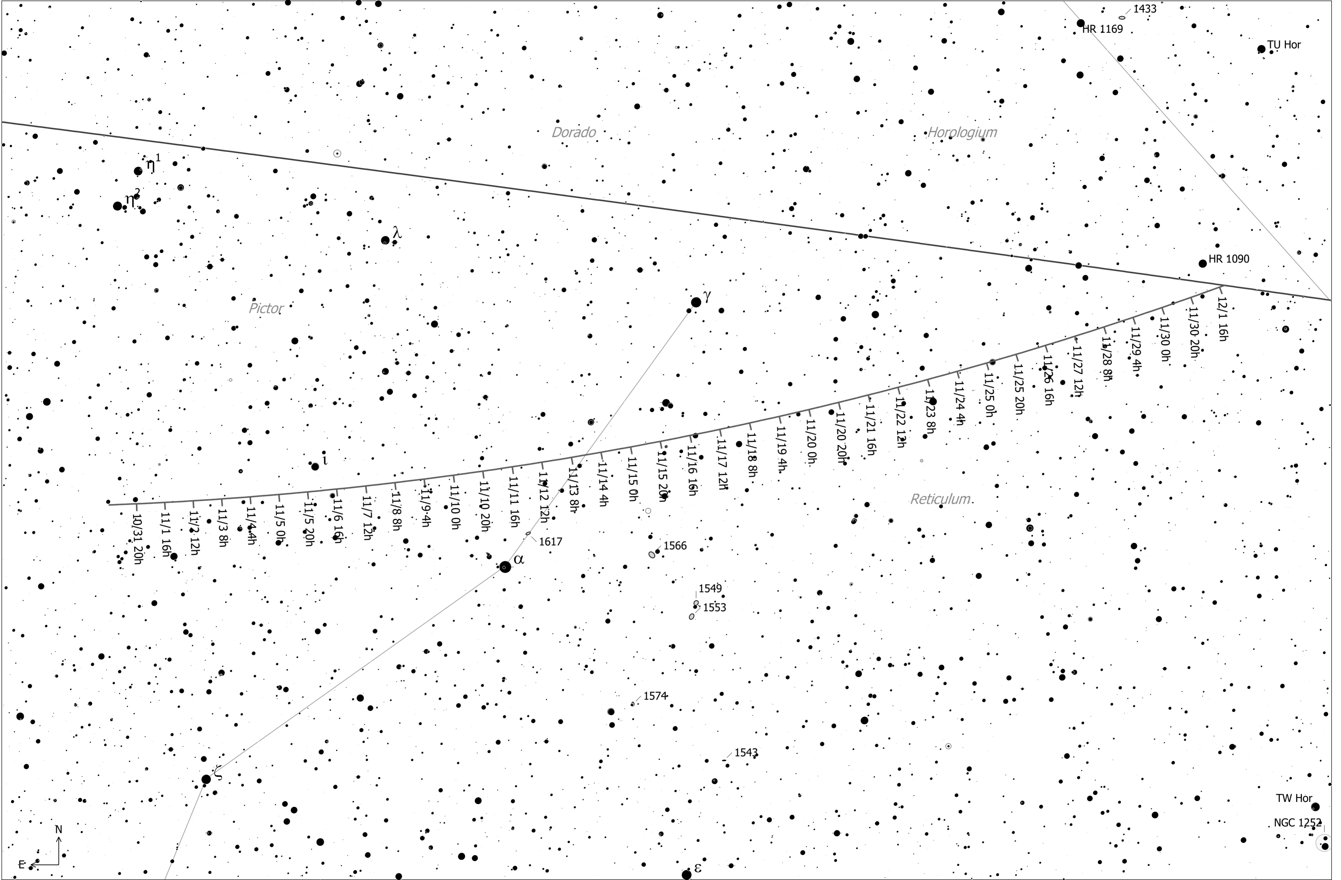
C/2020 Y2 (ATLAS) (Comet) Magnitude: 14.87 Coma Diameter: 38" SBr: 22.5 Mag/arcsec 2 Earth Distance: 3.0 AU
